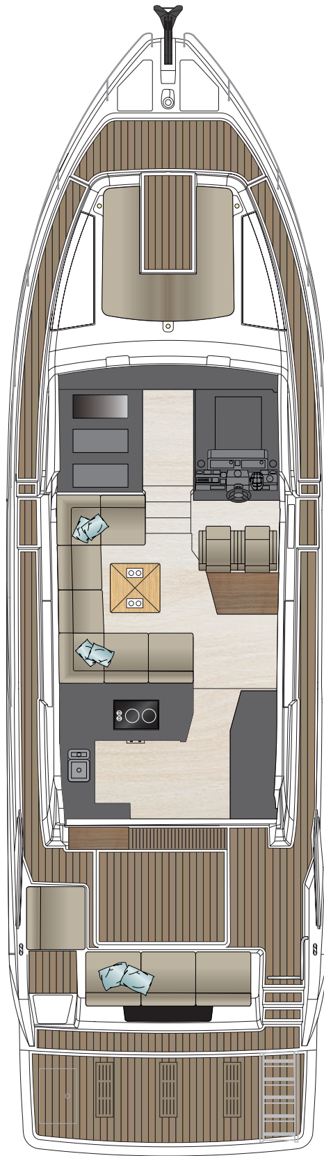
MAIN DECK
