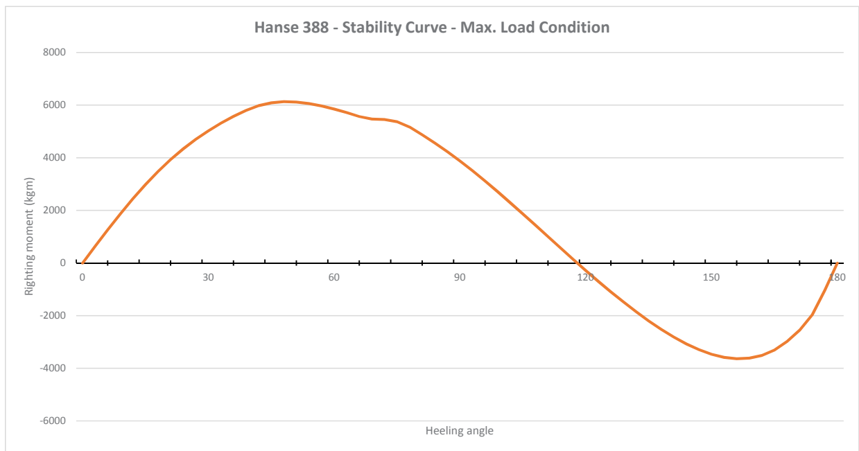
Hanse 388 - Medium draft keel, conventional rig
