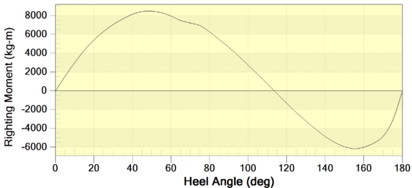
Righting Moment Curve
